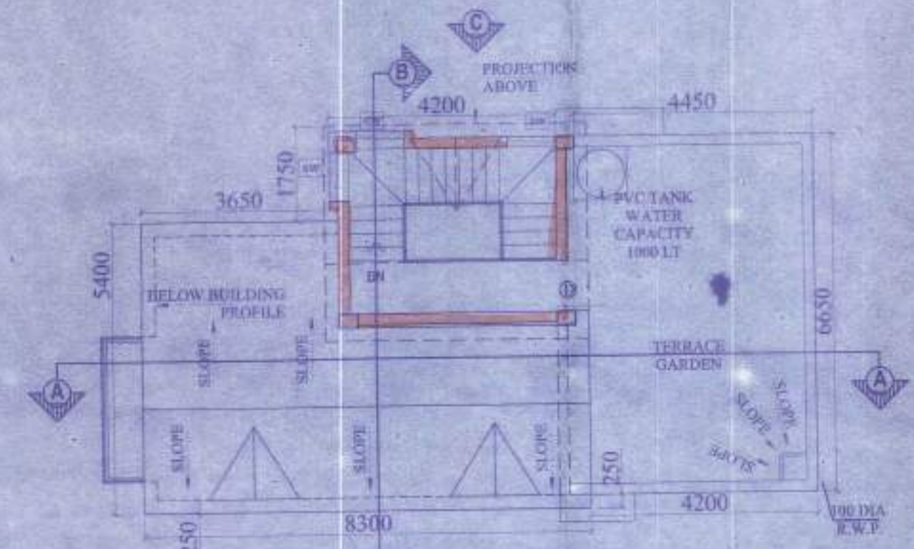
ROOF PLAN
