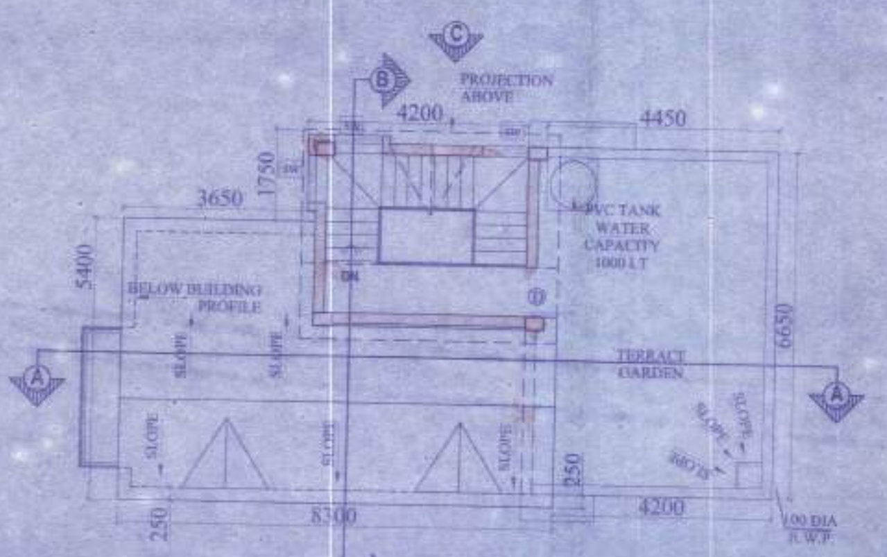
ROOF PLAN
